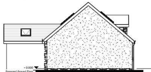
Proposed Side Elevation 1 : 100
